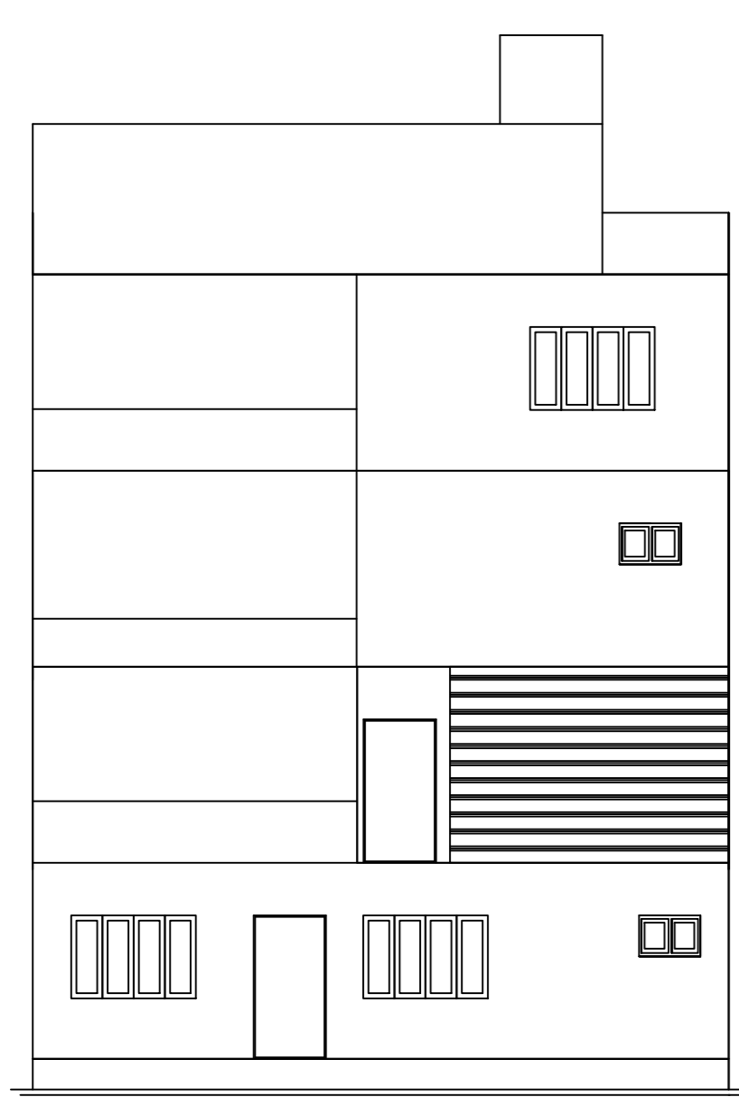
FRONT ELEVATION
